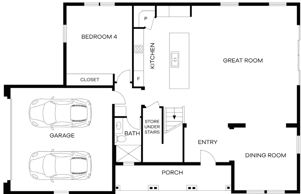
FIRST FLOOR
